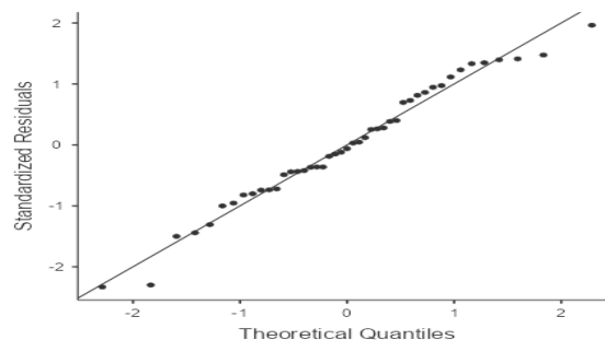
Gambar 1. Normal Q-Q Plot
