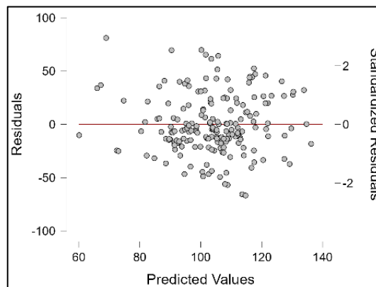
Gambar 3. Scatterplot
