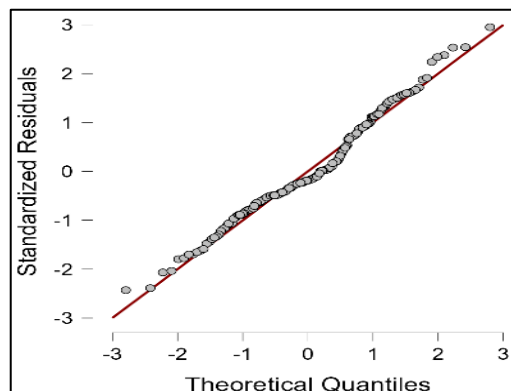
Gambar 2. q-q plot
