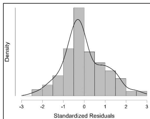
Gambar 1. Histogram
